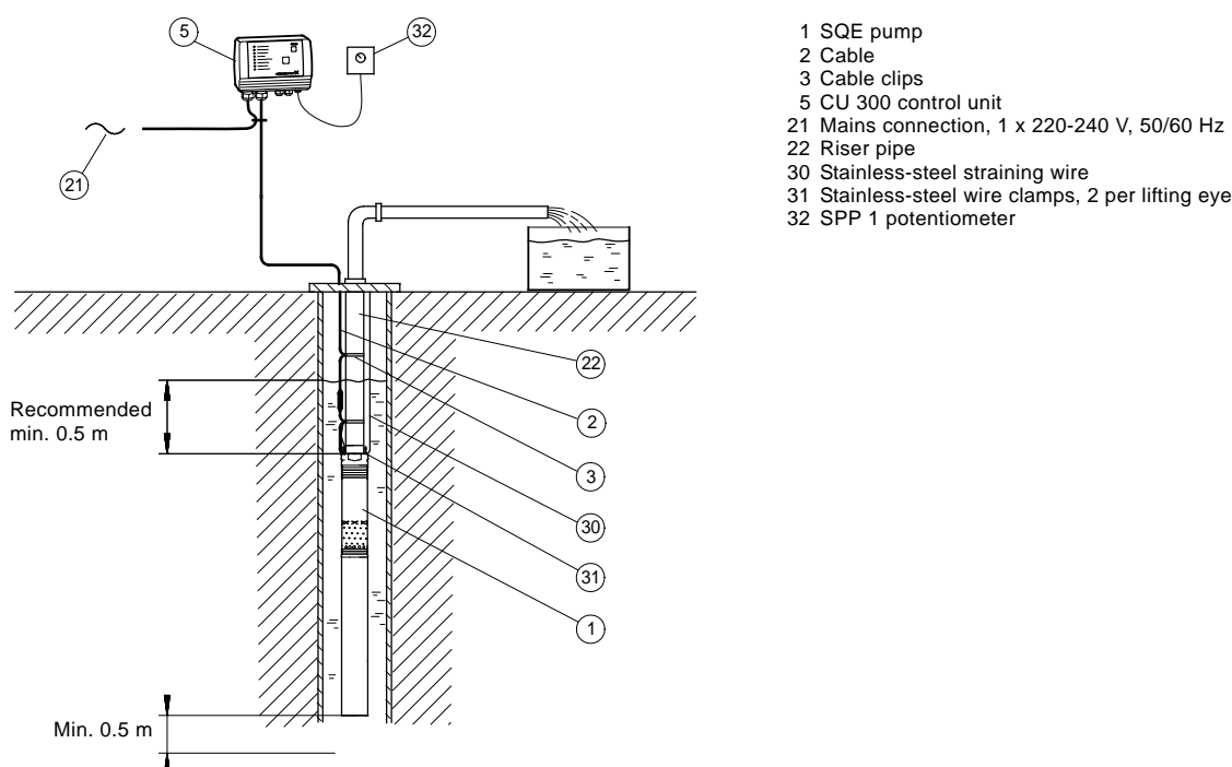
Fig. 15 Manual speed control of the SQE
